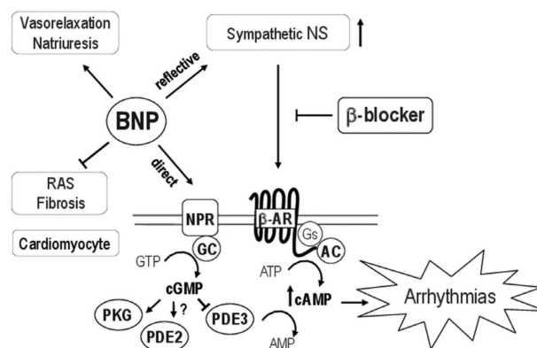
Figure 1 Schematic figure illustrating the brain natriuretic peptide (BNP)-dependent pathways and the possible interactions with beta blocker treatment. cGMP, cyclic guanosine monophosphate, NPR, natriuretic peptide receptor.
